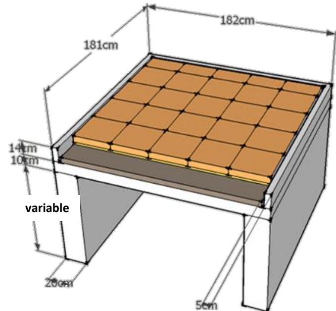
Dimensions of the base for a rounded shape
