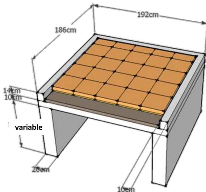
Dimensions of the base for a cubic shape
